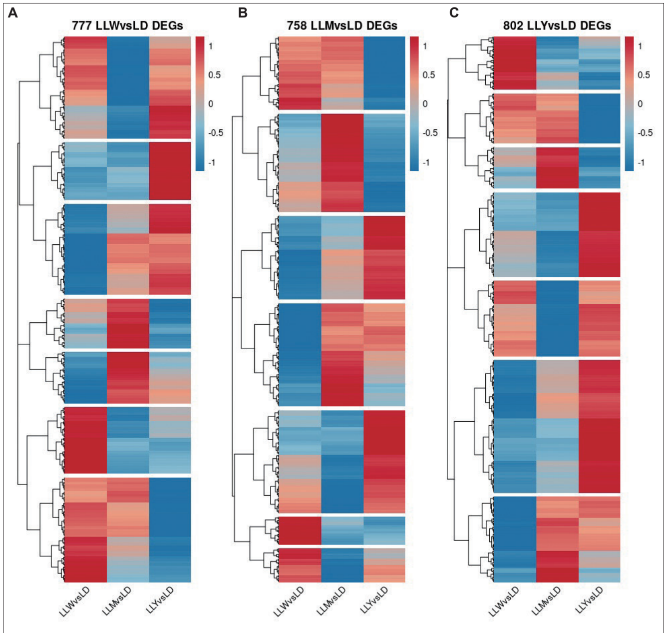
Supplementary Figure 4. Heatmap of all significant DEGs, from the point of view of 777 DEGs of LLW vs. LD with other contrasts (A); 758 DEGs of LLM vs. LD with other contrasts (B); and 802 DEGs of LLY vs. LD with other contrasts (C).
